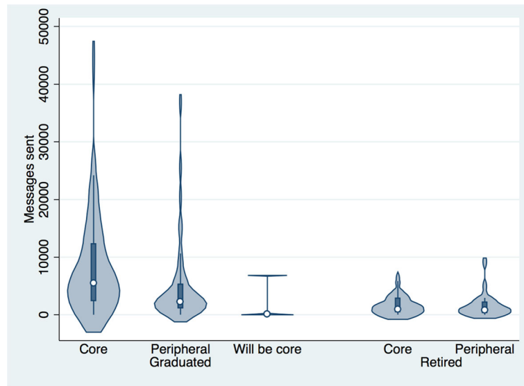
Fig. 2 Violin plot of total number of messages sent by project status and developer role
