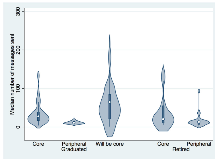
Fig. 3 Violin plot of median number of messages sent per developer by project status and developer role
